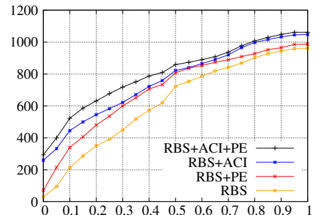
Figure 1: Coverage as a function of the fraction of RBS variables, |V^{\text{RBS}}|/|V| , in the first iteration of RBS that finds a real plan.
