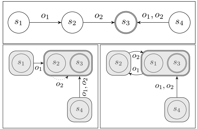
Figure 3: Concrete transition system \mathcal{T} (above) with abstractions \alpha_1 (bottom left) and \alpha_2 (bottom right) used in the proof of Theorem 3. Circles depict concrete states, abstract states are rounded rectangular, and abstract self loops are dotted.
